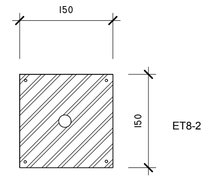
Brushed stainless steel mounting plate for ET-2-20DC
